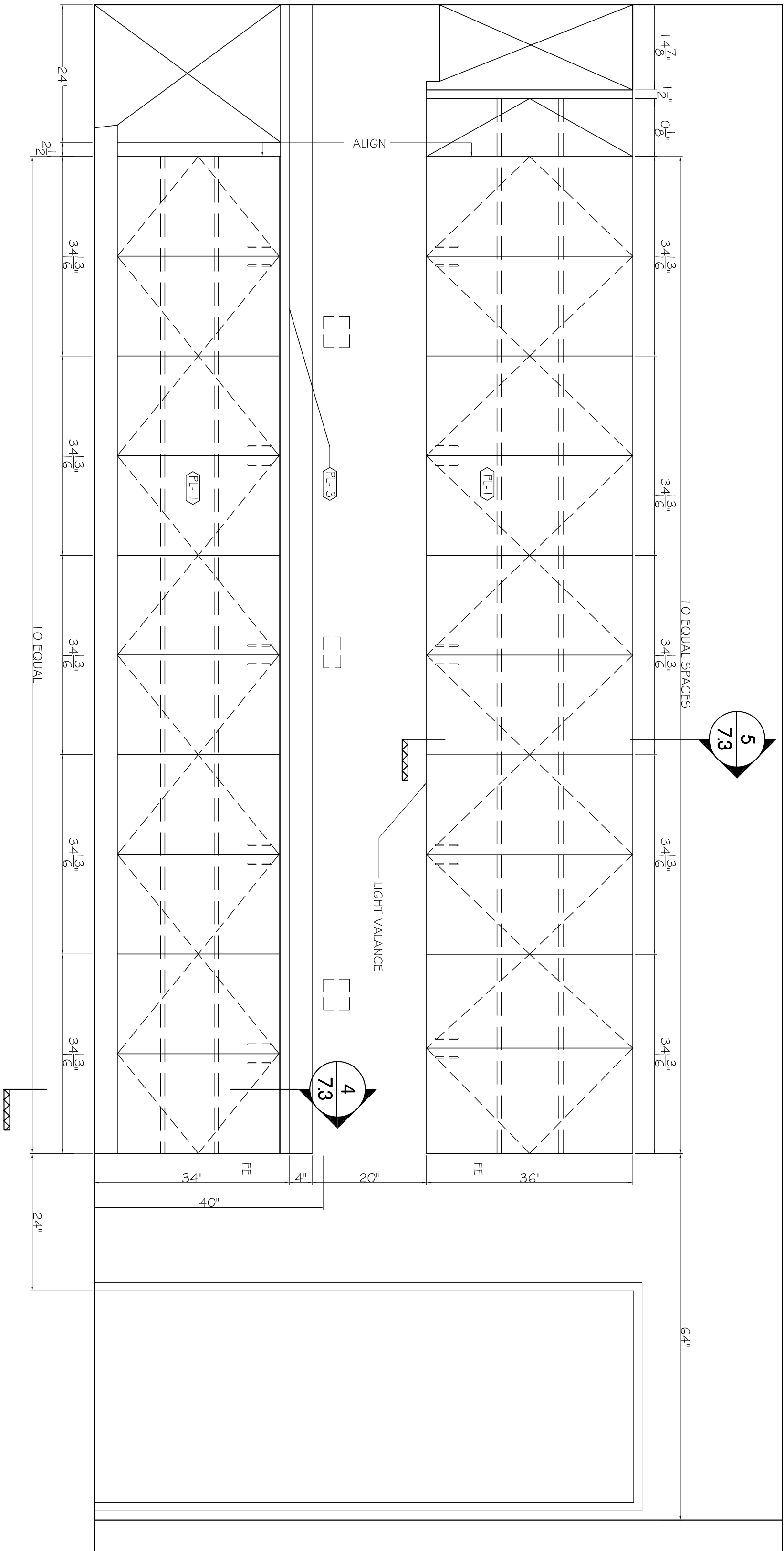
1 ELEVATION 7.0 3/4" = 1'
